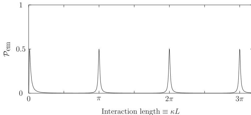
FIG. 3 – Photon emission probability in the cold atom regime ( k/\kappa = 0.01 ) for a mesa mode function.
